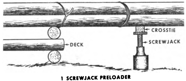
1 SCREWJACK PRELOADER
